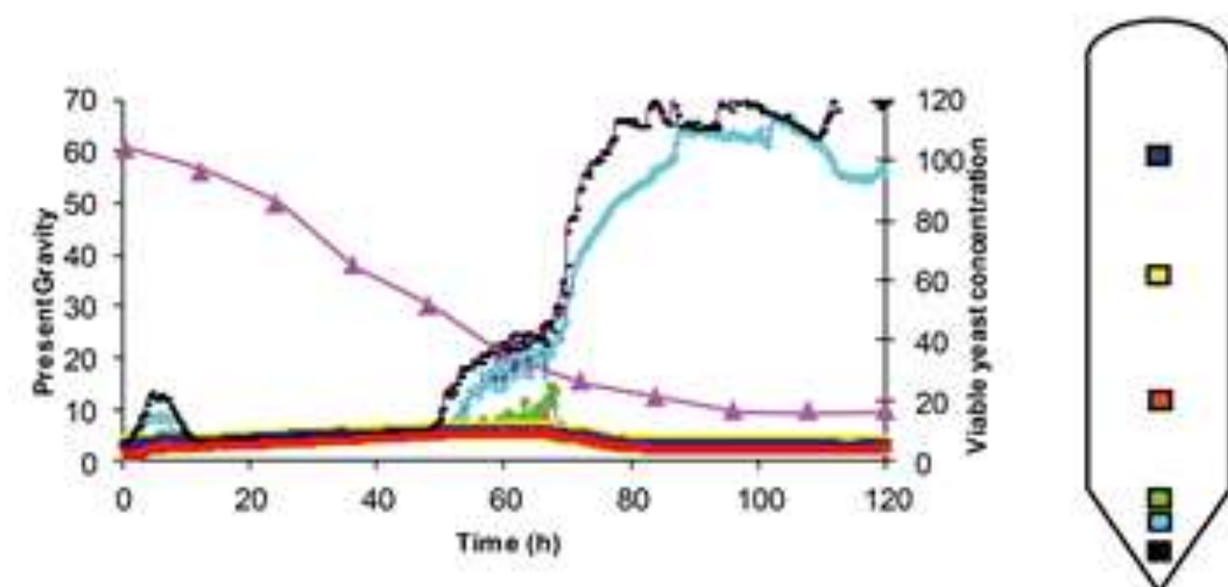
Figure 1. Actual measurements of viable yeast concentrations throughout a CCT during the course of a conventional (unmixed) fermentation, clearly illustrating the premature settling of yeast in the cone of the tank.
