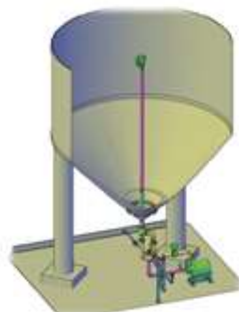
Figure 2. Dynamic fermentation system utilizing rotary jet mixing with bottom-entry installation. Liquid is circulated from the tank outlet through a centrifugal pump to the mixer, which distributes the incoming liquid to all areas of the tank. The system is installed through the tank swing cone and bottom outlet flange, minimizing necessary tank modification.
