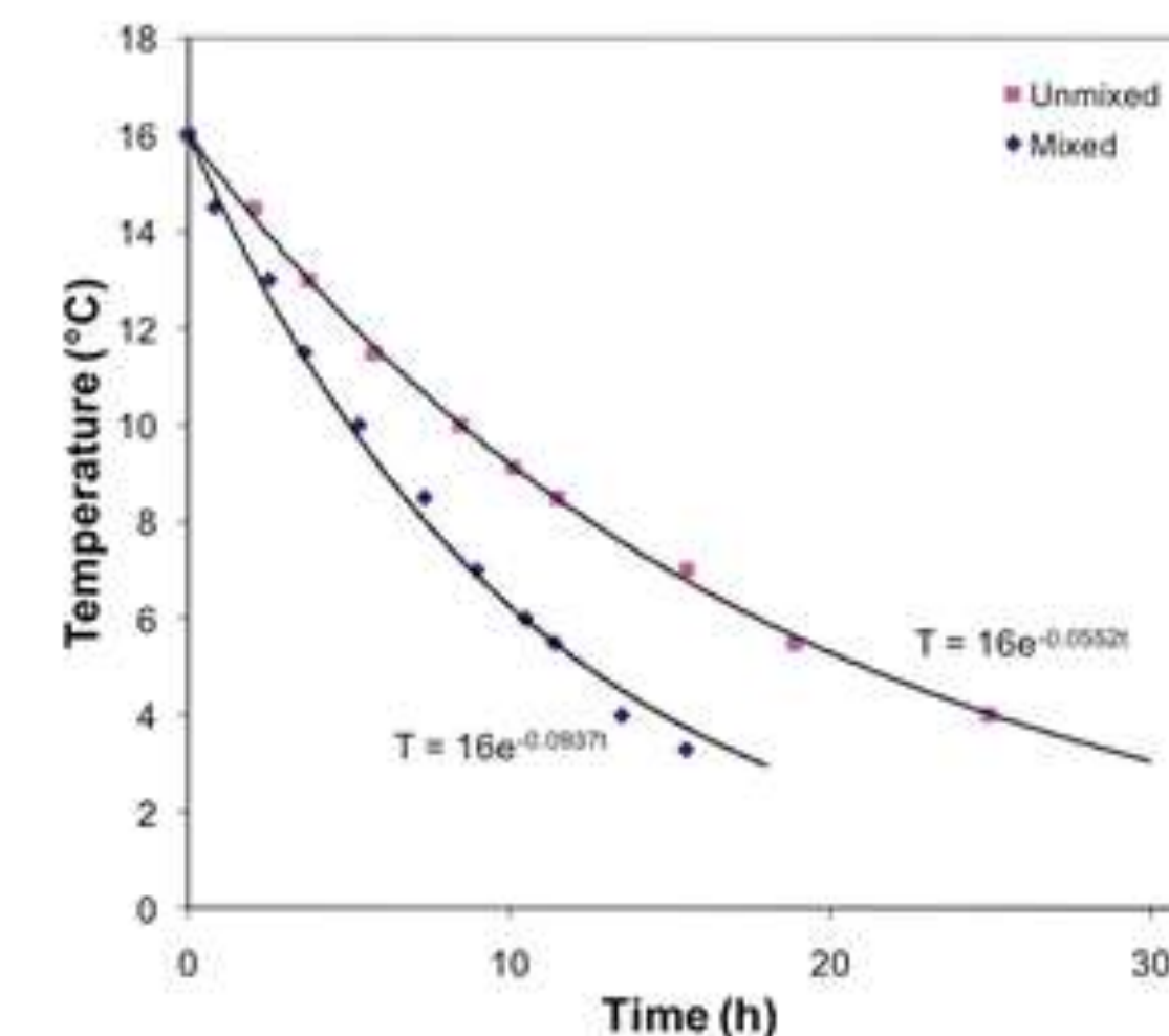
Figure 4. Effect of mixing on cooling time in an 1800 hL CCT.
